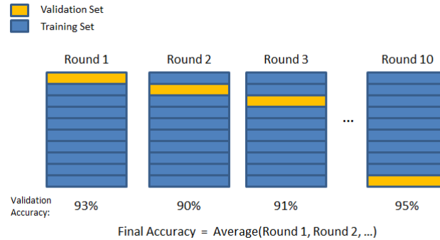
Crossvalidation
