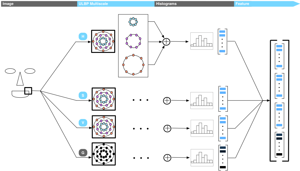
FIGURE 3.2: Implemented System.
