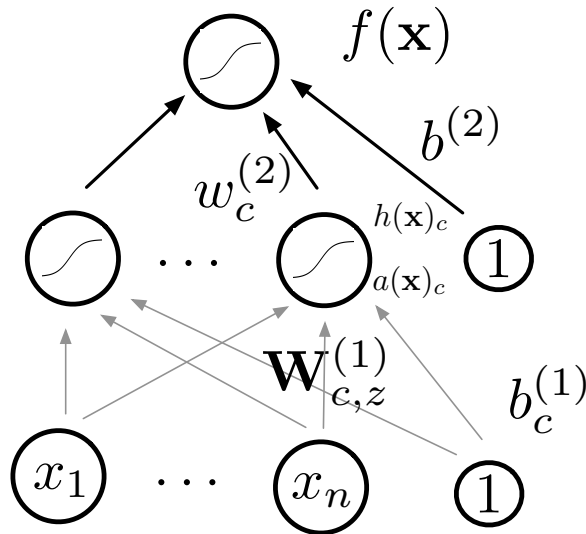
FIGURE 10.4: Single-layer Network.
