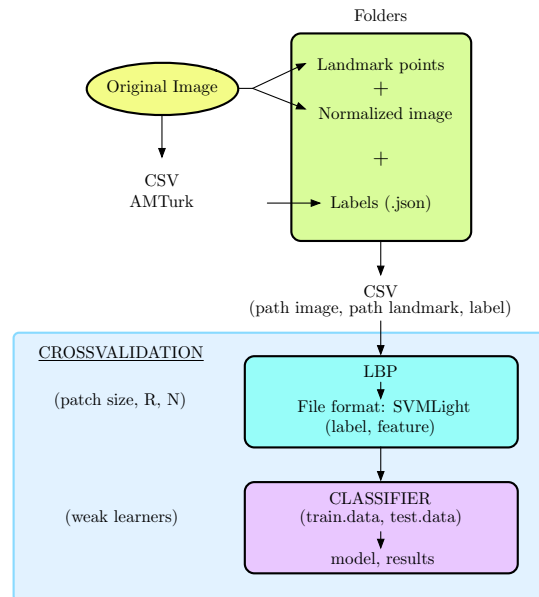
FIGURE 3.6: Implementation Hints.
