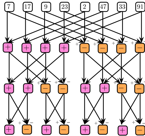
FIGURE 4.1: Fast Walsh Hadamard.
