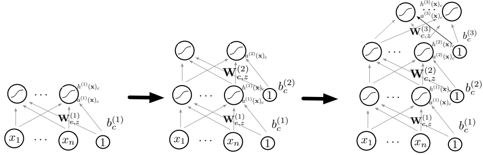
FIGURE 10.8: Pretraining.
