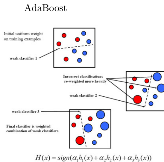
FIGURE 3.4: Adaboost.
